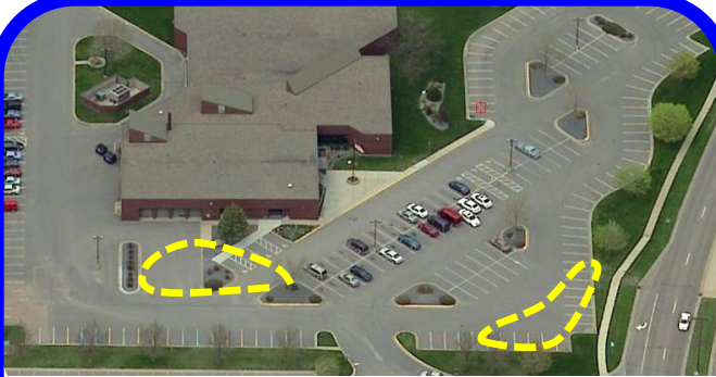
Unused parking was removed to reduce impervious area and provide bioretention cell locations.
